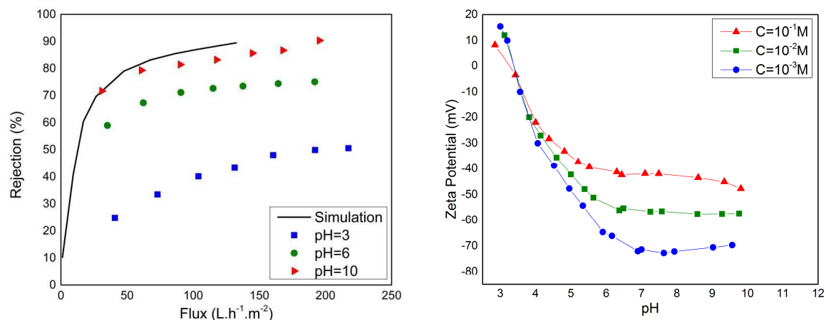
Figure 9. Ion rejections as a function of permeate flux for 10^{-2} M NaCl feed at various pH (left). Solid curves are simulation obtained with ROSA and dots the experimental results. Zeta potential of the NF270 membrane surface as a function of pH and KCl concentration (right).
