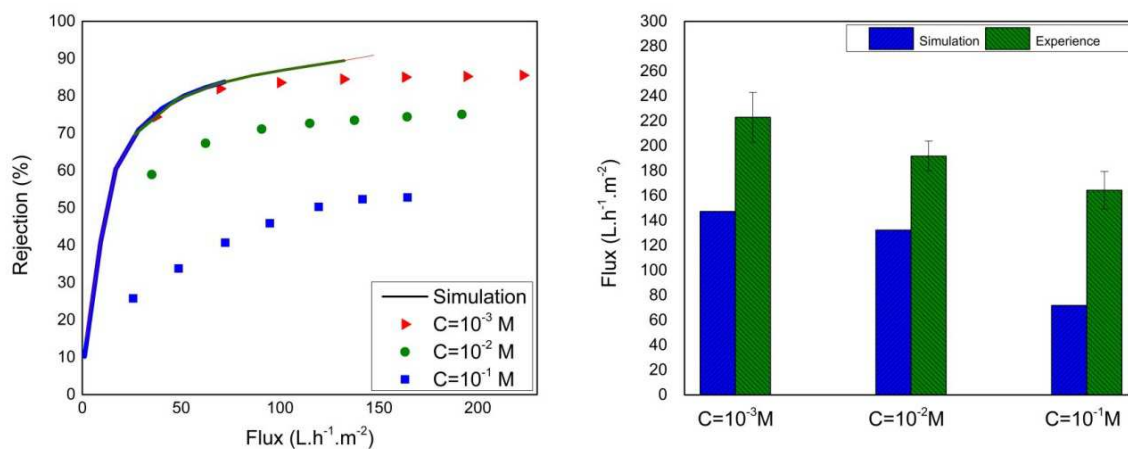
Figure 8. Comparison between simulated and experimental ion rejections as a function of permeate flux for different NaCl feed concentration at pH 6 (left) and the corresponding permeate flux as a function of NaCl feed concentration (right). Solid curves are simulation results obtained with ROSA and symbols the experimental results.
