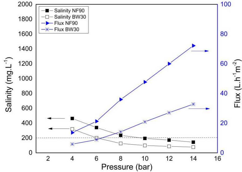
Figure 5. Effect of pressure on permeate flux and salinity for filtration of Feed 3 using the NF90 and BW30 membranes. The dashedline represents the lower limit of Tunisian salinity norm.
