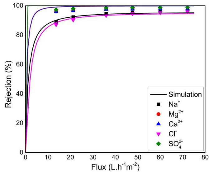
Figure 11. Ion rejections as a function of permeate flux for Feed 3 nanofiltered by NF90. Solid curves are simulation results obtained with Nanoflux ® and symbols the experimental results.
