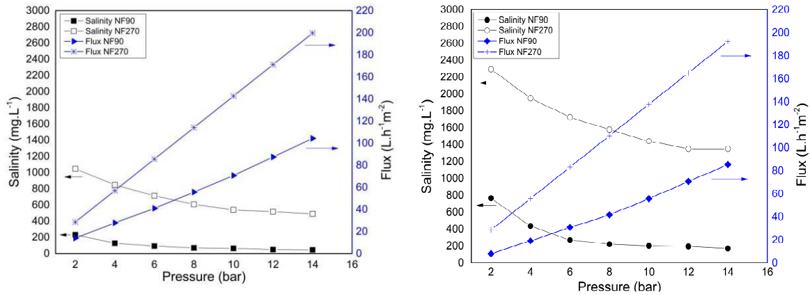
Figure 3. Effect of pressure on permeate flux and salinity for filtration of Feed 1(left) and Feed 2 (right) using the NF90 and NF270 membranes.
