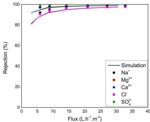
Figure 6. Ion rejections as a function of permeate flux for Feed 3 treated with BW30. Solid curves are simulation results obtained with ROSA and symbols the experimental results.
