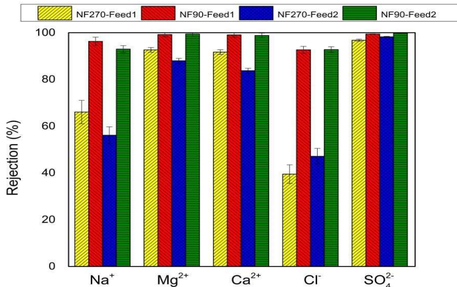
Figure 4. Rejection of monovalent and bivalent ions by NF270 and NF90 membranes at a fixed trans-membrane pressure of 10 bar for Feed 1 and Feed 2.
