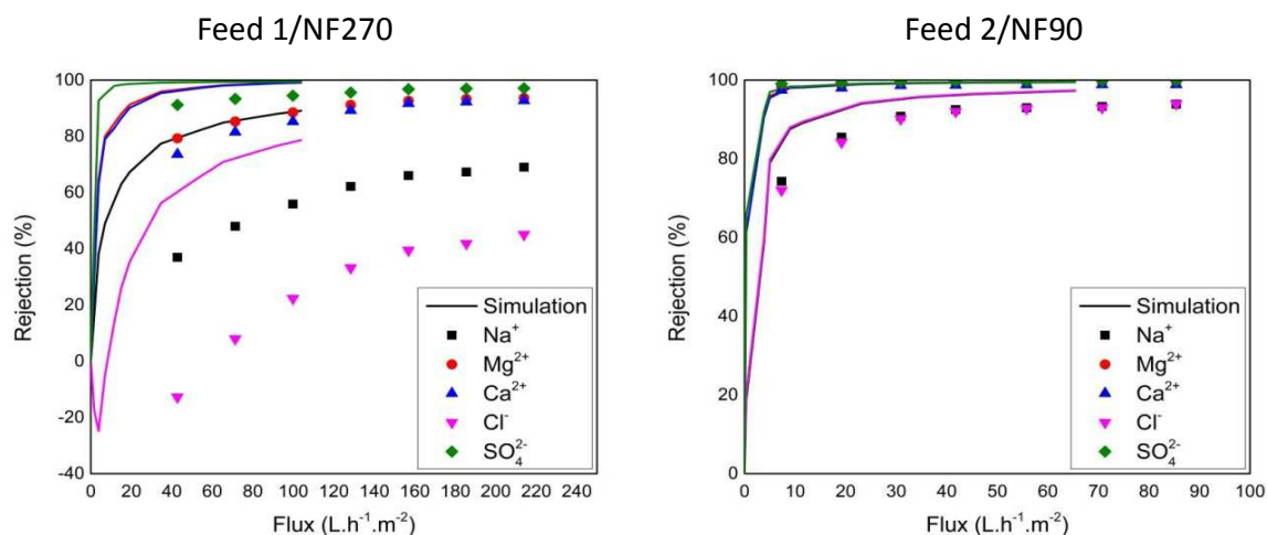
Figure 7. Ion rejections as a function of permeate flux for Feed 1/NF270 (left) and Feed 2/NF90 (right). Solid curves are simulation obtained with ROSA and symbols the experimental results.
