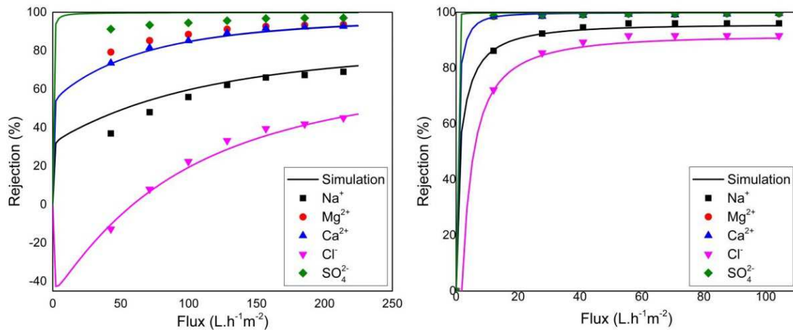
Figure 10. Ion rejections as a function of permeate flux for Feed 1 nanofiltered by NF270 (left) and by NF90 (right). Solid curves are simulation results obtained with Nanoflux ® and symbols the experimental results.
